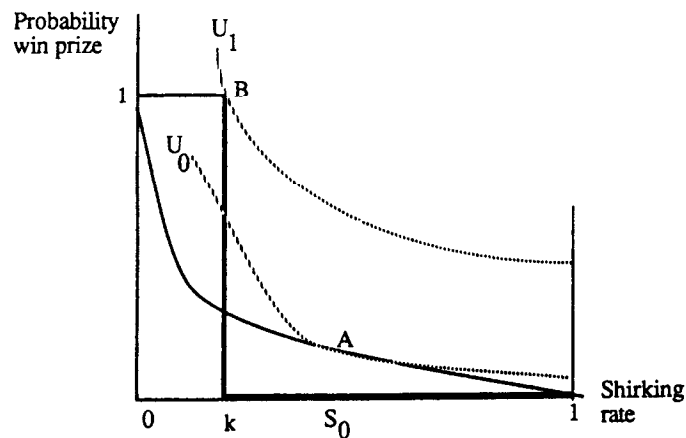
Fig. 3. Perfect information reduces shirking ( S_0 > k ).
