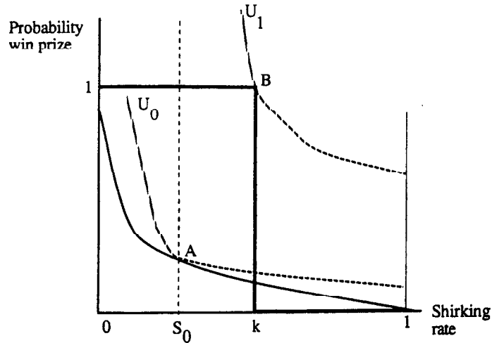
Fig. 2. Perfect information increase shirking ( S_0 < k ).
